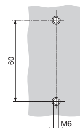
Mounting with mounting angle
