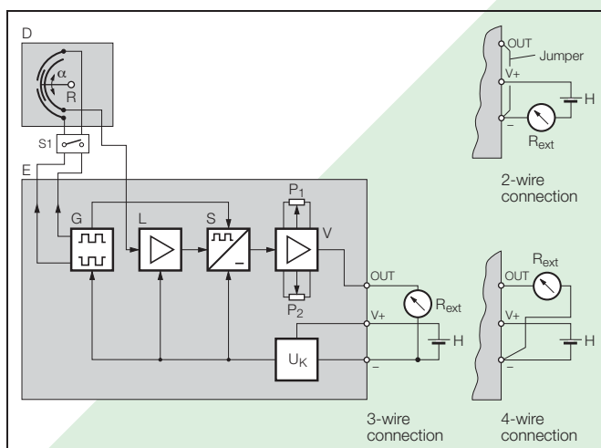
Fig. 4. Block diagram
