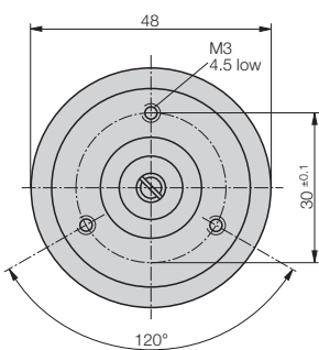
Fig. 9. KINAX 3W2 with shaft dia. 1/4", length 12 mm.
