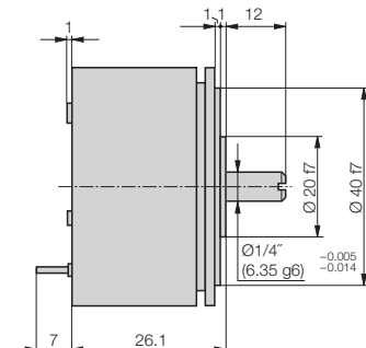
Fig. 9. KINAX 3W2 with shaft dia. 1/4", length 12 mm.
