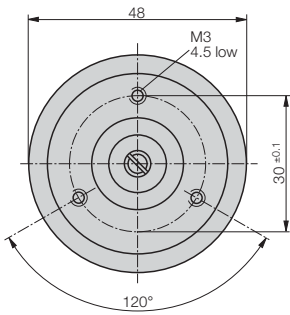
Fig. 7. KINAX 3W2 with shaft dia. 2 mm, length 12 mm.
