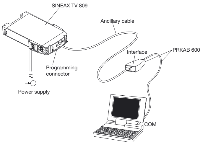
Fig. 6. Configuring a SINEAX TV 809, Ex version.
