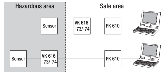
Fig. 10. Configuring the SINEAX VK 616, types 616-73/74 when the transducer and/or the sensor are in the hazardous are.
