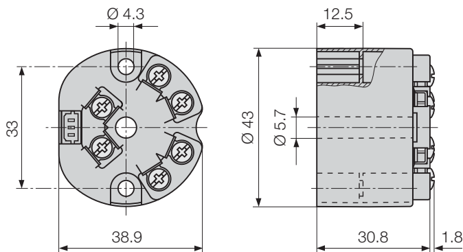
Fig. 14. SINEAX VK 616-72/74, electrically isolated.
